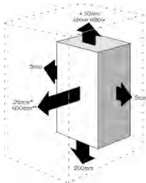
*600mm service clearance required to a fixed surface (**25mm from removable door or panel)
