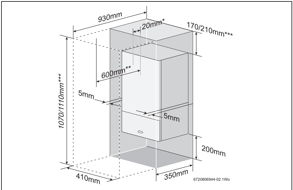
Fig. 11 Unventilated compartment
