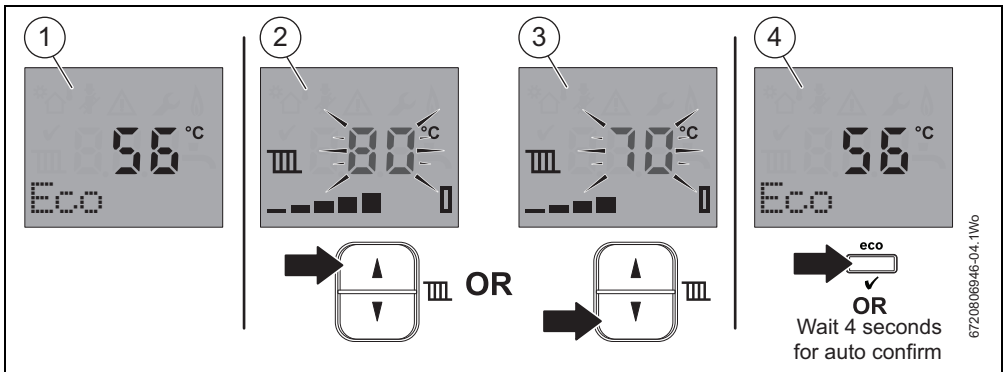
Fig. 4 Adjust appliance flow temperature
