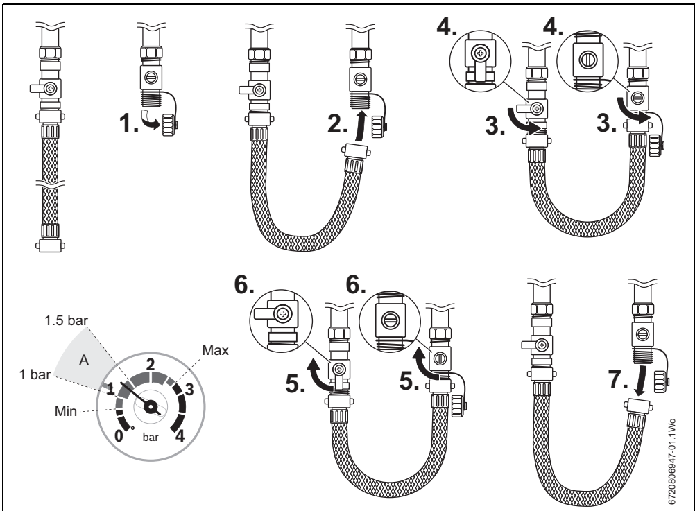
Fig. 10 External filling loop
